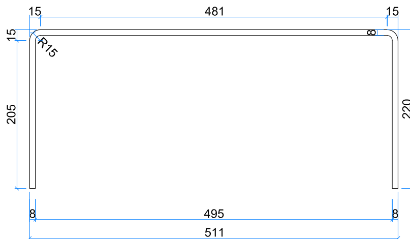
VISTA FRONTAL
